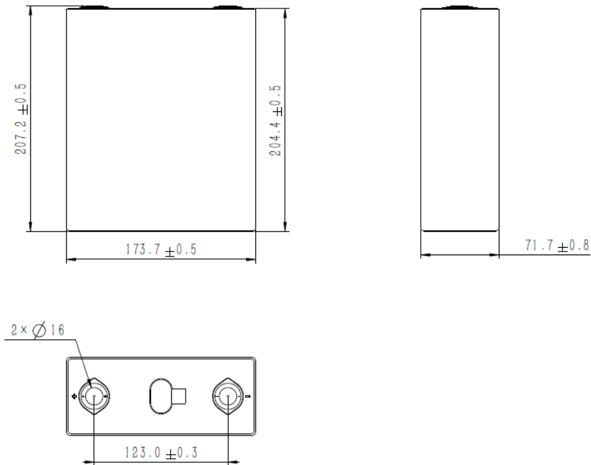
Fig.7 Diagram of Cell Size and Appearance
